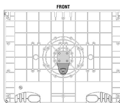
T10-380 / T10-385 / T10-390 Round Rail Mount
