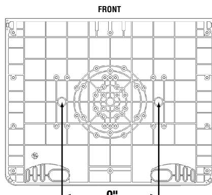
T10-521 / T10-526 Socket Mount, T10-540 Square Rail Mount installation dimension
